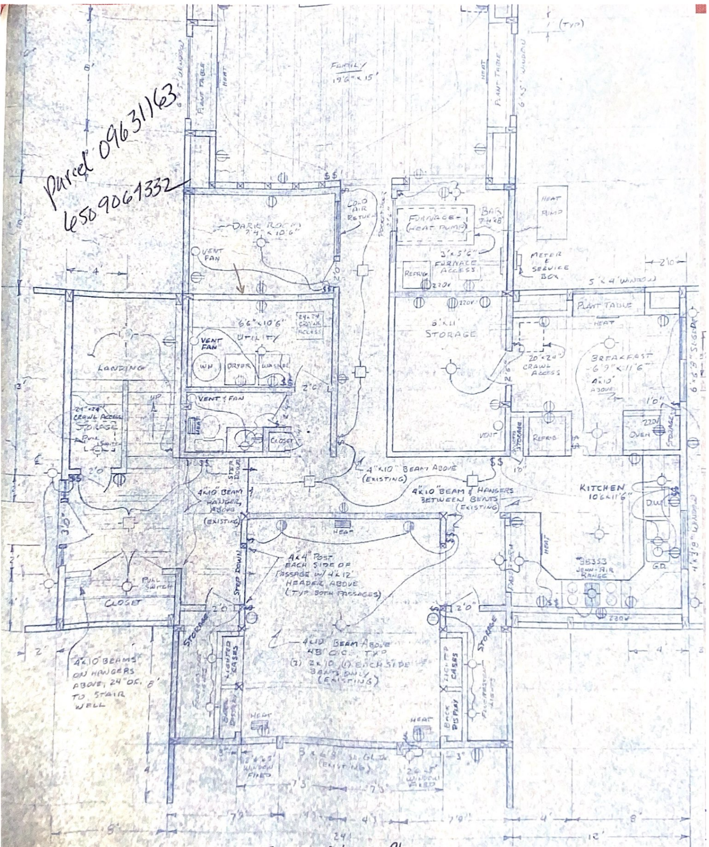
First Floor Plan FIRST FLOOR PLAN
