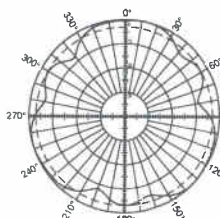
Horizontal pattern ±45°-polarization 1945 MHz
