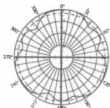
Horizontal pattern ±45°-polarization 1945 MHz
